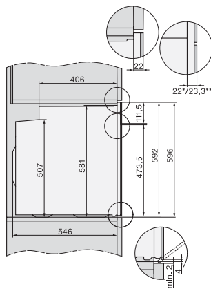
Side view H 7000, installation drawings
