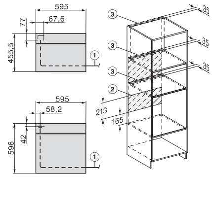
Installation, combination with H 7000 BM, installation drawings
