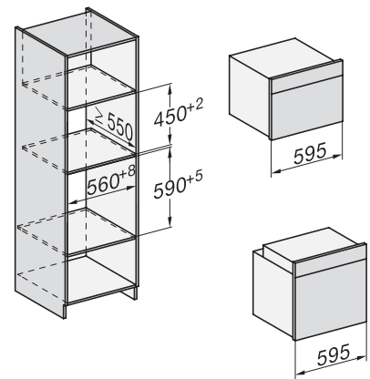
Installation with H 7000 BM, installation drawings
