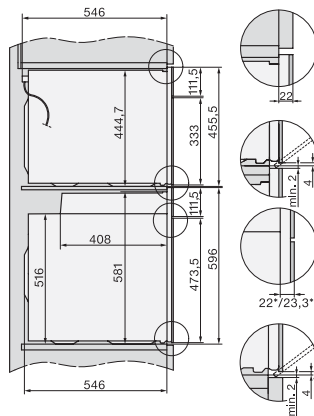
Side view, combination with H 7000 BM, installation drawings
