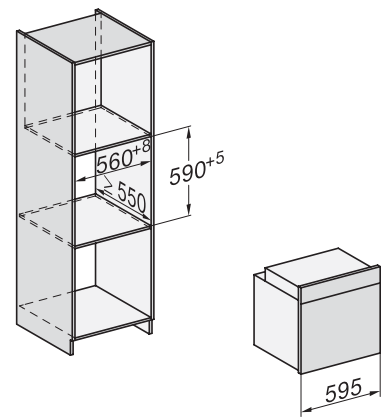
Built-in H 7000, installation drawings
