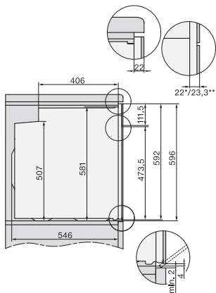
Side view H 7000 under bench, installation drawing
