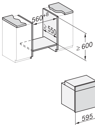
Installation H 7000 underframe, installation drawings
