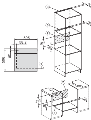
H 7000, installation drawing
