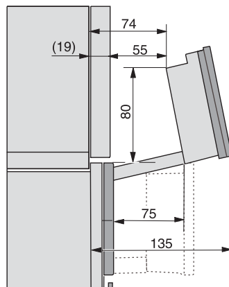
Motorised lift-up control panel, installation drawings
