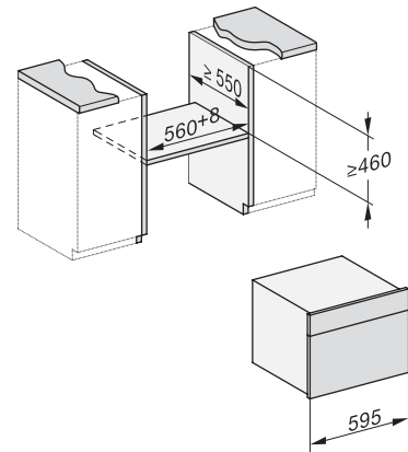
Built-under, installation drawing
