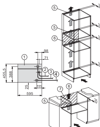
Installation, installation drawing,
