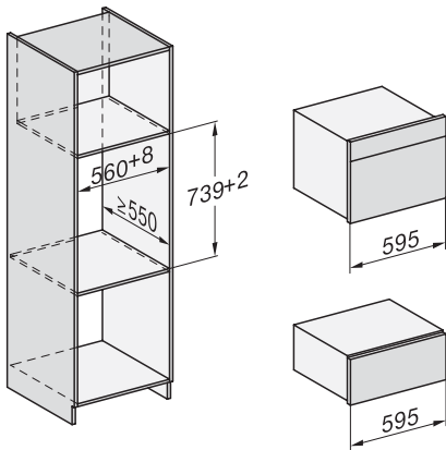
Installation, with ESW7020, installation drawings
