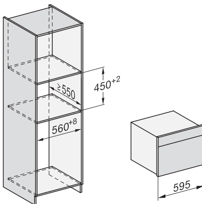
Built-in tall cabinet, installation drawing
