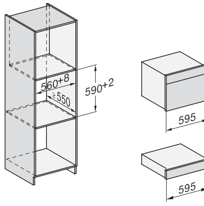
Installation, with ESW7010, installation drawings
