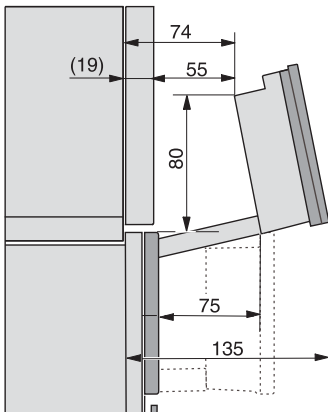
Motorised lift-up control panel, installation drawing
