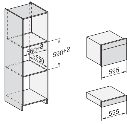
Installation, with ESW7x10, installation drawings
