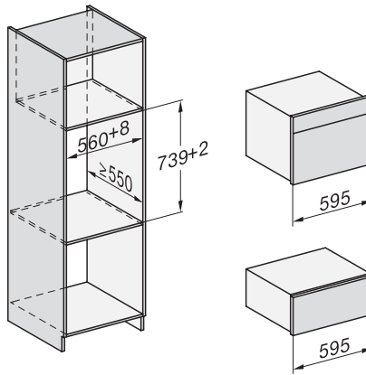
Installation with, ESW7x20 installation drawings
