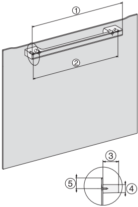
Handle, glass, installation drawings 1) 400 mm, 2) 360 mm, 3) 47 mm, 4) 27 mm, 5) 32.5 mm
