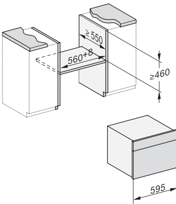
Built-under, installation drawing drawing
