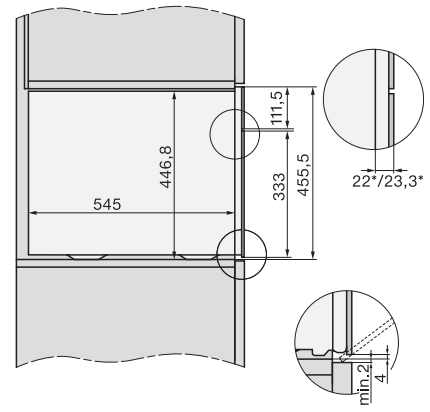
Side view, installation drawing 22 mm glass
