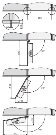
CVA 7000, top view (installation drawing)
