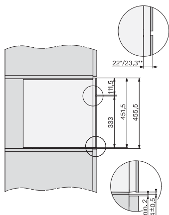
CVA 7000, side view (installation drawing) 22 mm – glass
