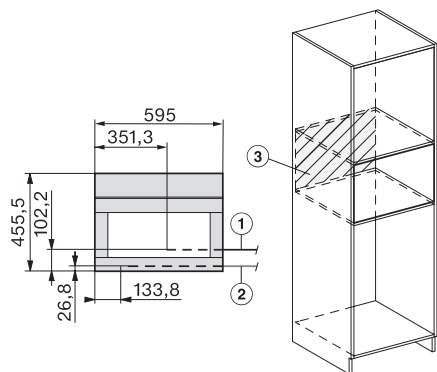
CVA 7000, connection details (installation drawings)
