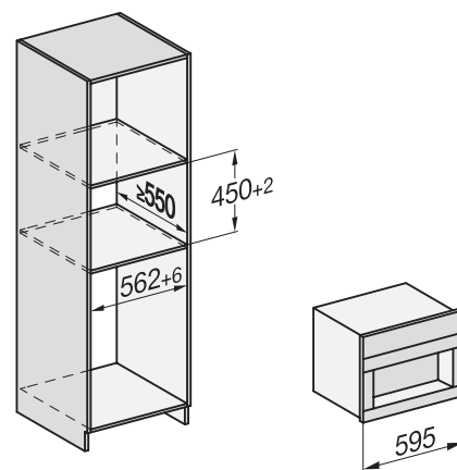
CVA 7000, isometric view (built in)
